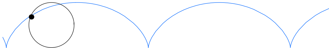
Figure 5. A Cycloid.
